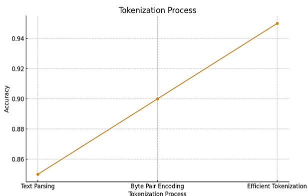
Figure 3: Tokenization Process
