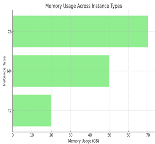
Figure 8: Memory Usage Across Instance Types
